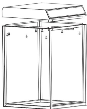
Step 4: Screws * 8
