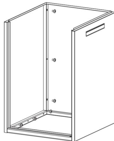
Step 3: Screws * 6
