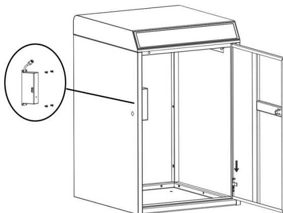
Step 5: Door Pin * 1 Screws to install the lock Body * 4
